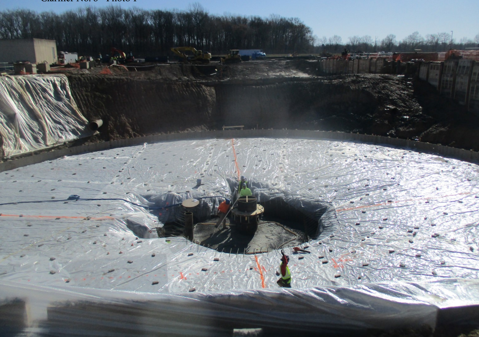
Clarifier No. 8 - Photo 1
